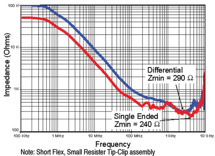
Figure 6: Typical differential input impedance verses frequency
