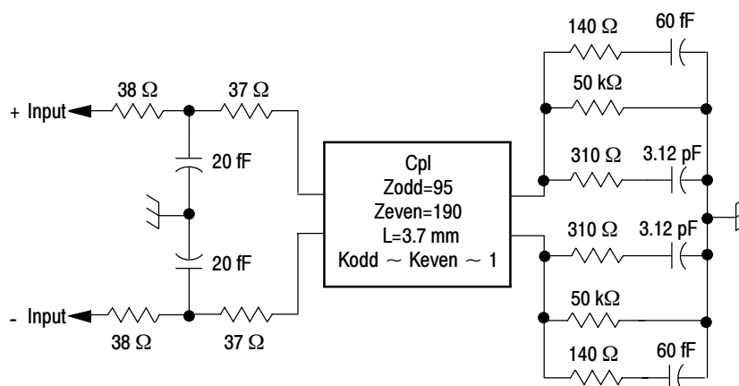
Figure 3: Typical probe input model
