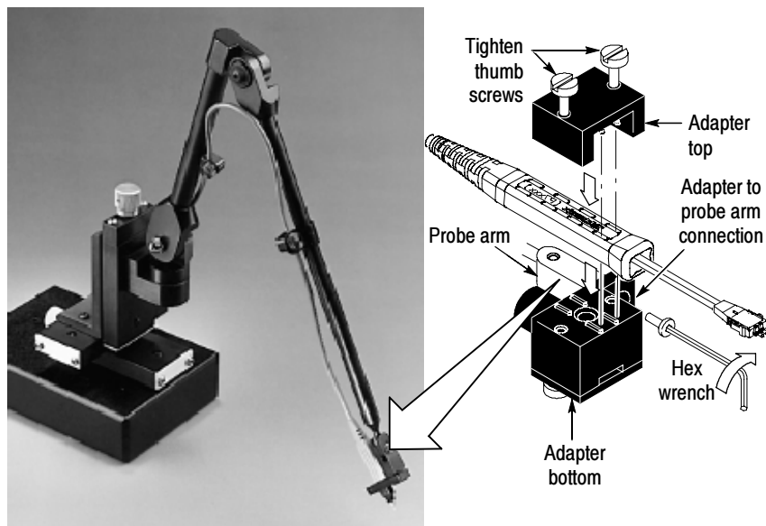
Figure 10: Adapter fixture
